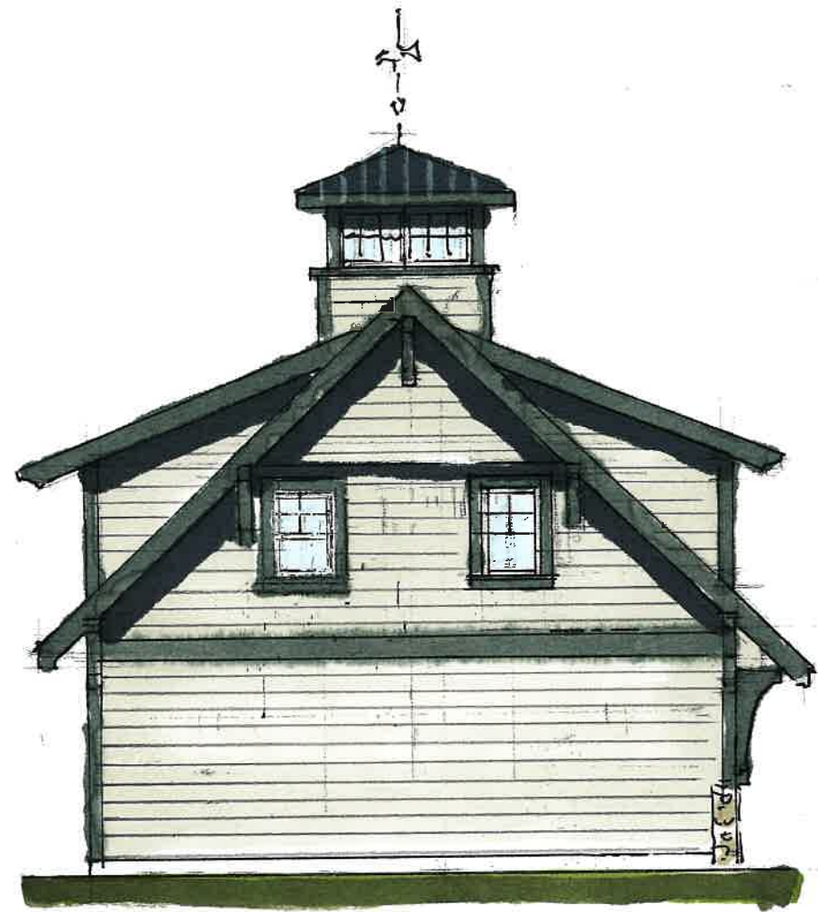
NORTH ELEVATION STOKER CARRIAGE HOUSE
